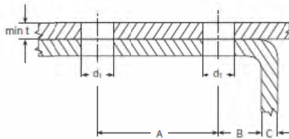
FIGURE 2—INSTALLATION INSTRUCTIONS
