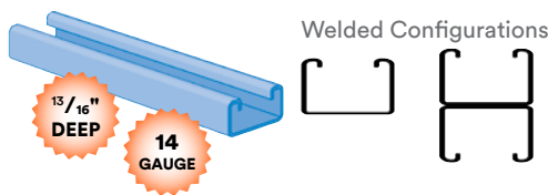
Welded Configurations
