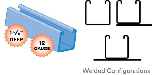
Welded Configurations
