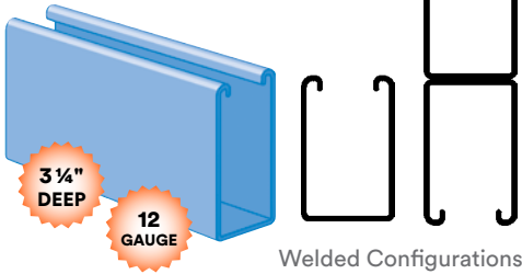
Welded Configurations
